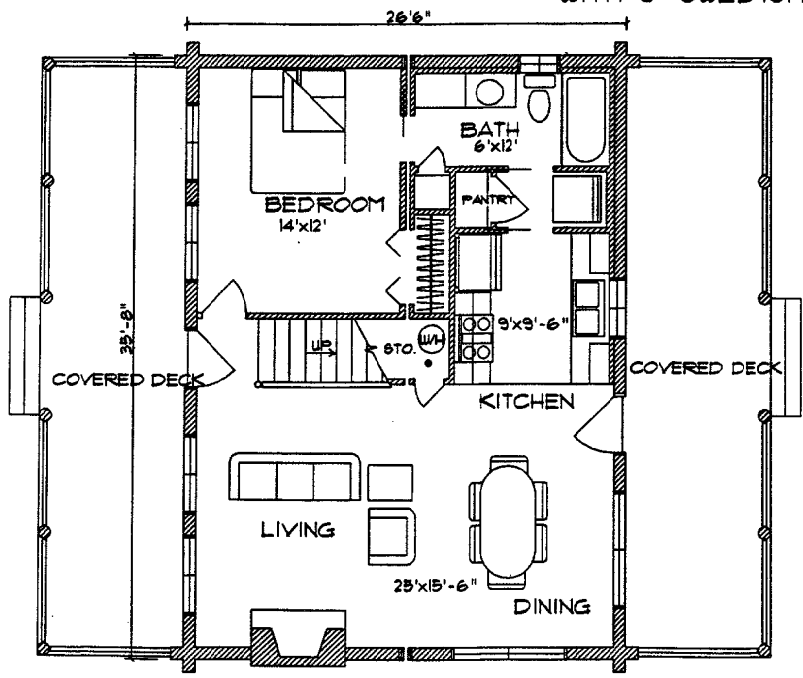
MAIN FLOOR PLAN 856 SQ. FT.
