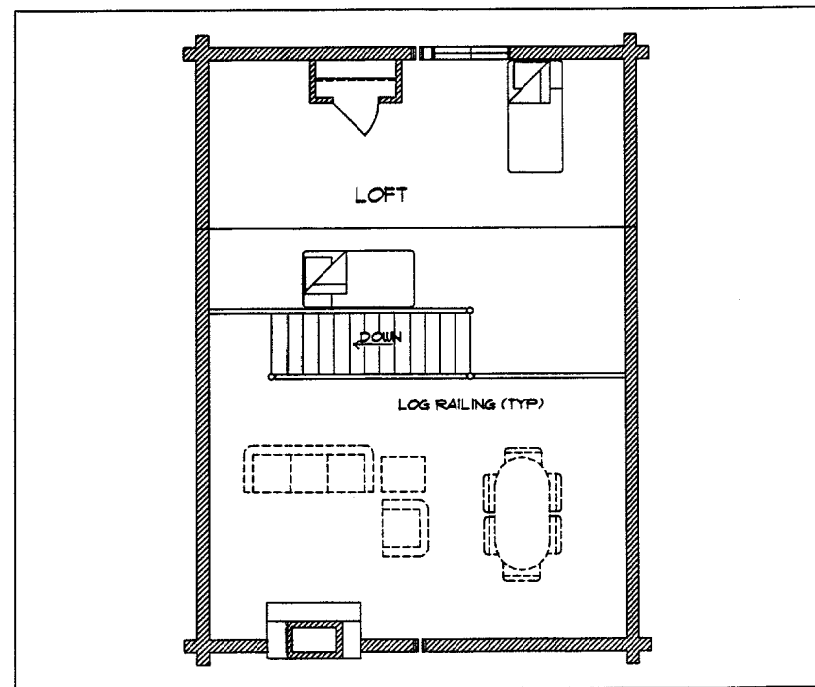
UPPER FLOOR PLAN 425 SQ. FT.
