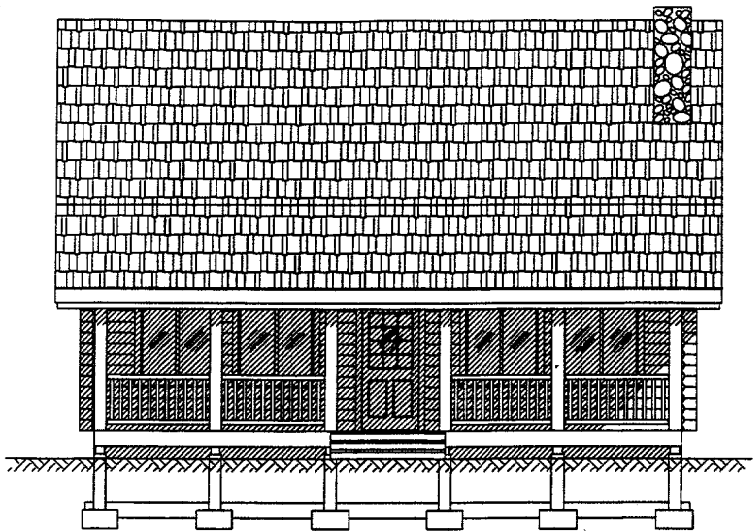
FRONT ELEVATION
